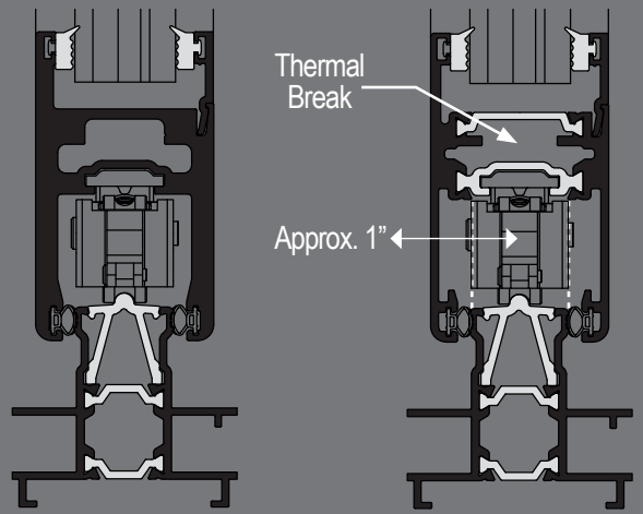
Non-Thermally Broken Panel Detail
