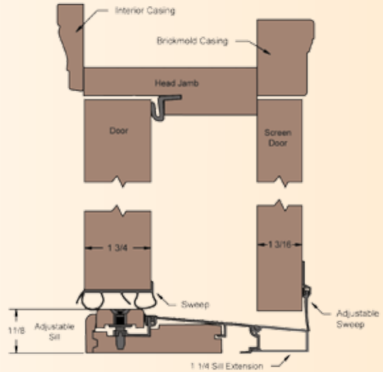
Non-Impact Prehang Details with Standard Jamb and Inswing Sill and Storm Door Attached
