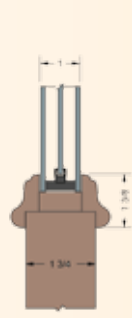
Raised Molding 1" I.G.
