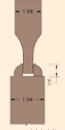
Recessed Molding W/ Standard Panel
