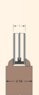
Recessed Molding 1" I.G.
