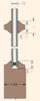
Recessed Molding Style B & 1" SDL Bar
