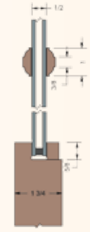
Mission Molding & 1" SDL Bar
