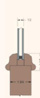
Raised Molding 1/2" I.G.
